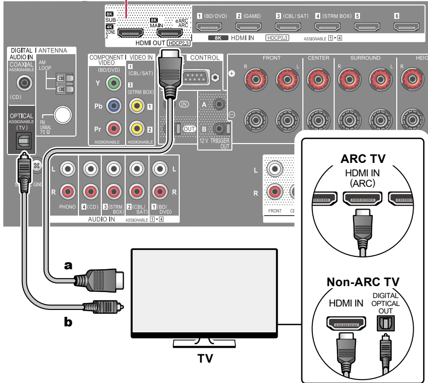
a HDMI cable, b Digital optical cable
