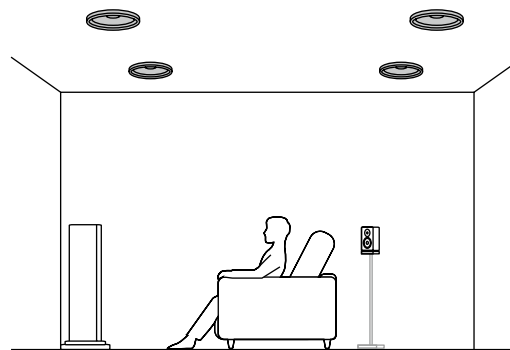
5.1.4 ch (Top Front and Top Rear) ( →p36)
